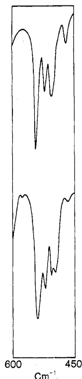
Figure 4. Infrared spectra in the region 450\text{--}600\text{ cm}^{-1} of \text{Me}_3\text{SnONPhCOPh} in the solid state (upper) and in dichloromethane solution (lower).
