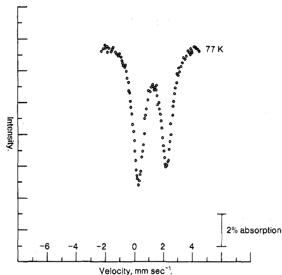
Figure 2. The tin-119m Mossbauer spectrum of Ph 3 SnONPhCOPh run at 77°K vs. a Ba 119m SnO 3 source.
