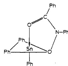
Figure 1. The structure of O -(triphenylstannyl)- N -phenyl- N -benzoylhydroxylamine.
